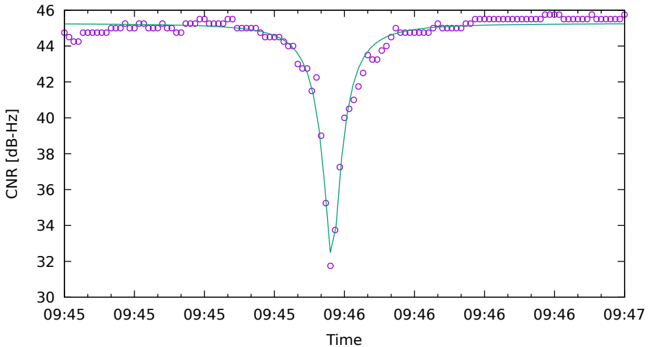
CNR fit for C05 on SamsungS20 - drive 4 (DOY263)
