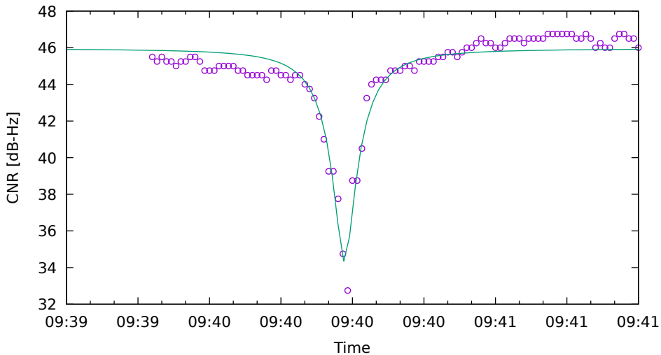
CNR fit for C12 on SamsungS20 - drive 1 (DOY263)
