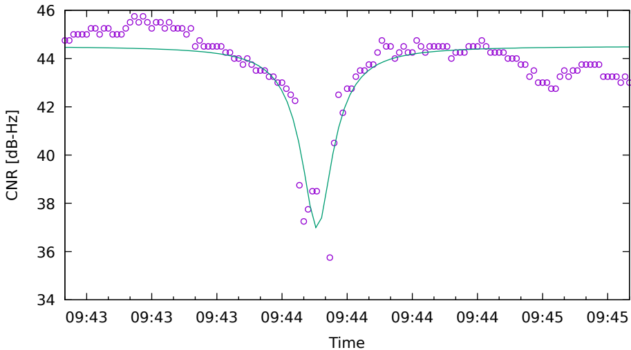
CNR fit for C12 on SamsungS20 - drive 3 (DOY263)
