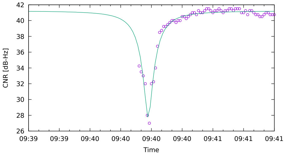
CNR fit for C16 on SamsungS20 - drive 1 (DOY263)
