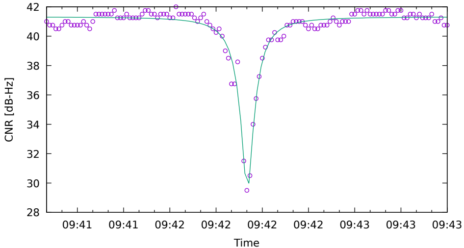
CNR fit for C16 on SamsungS20 - drive 2 (DOY263)
