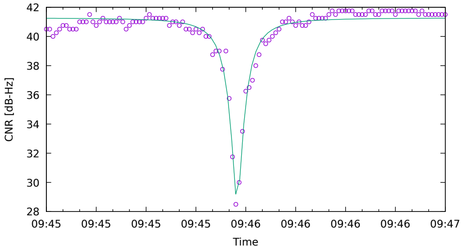
CNR fit for C16 on SamsungS20 - drive 4 (DOY263)
