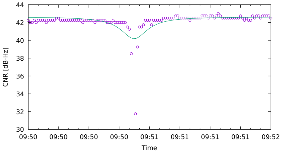
CNR fit for C16 on SamsungS20 - drive 7 (DOY263)
