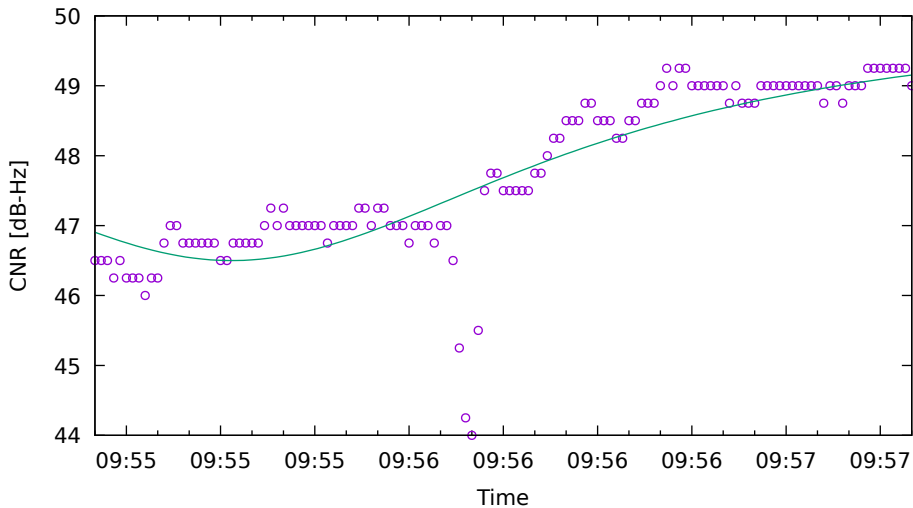
CNR fit for C34 on SamsungS20 - drive 10 (DOY263)
