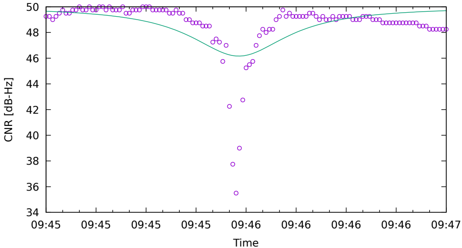
CNR fit for C34 on SamsungS20 - drive 4 (DOY263)
