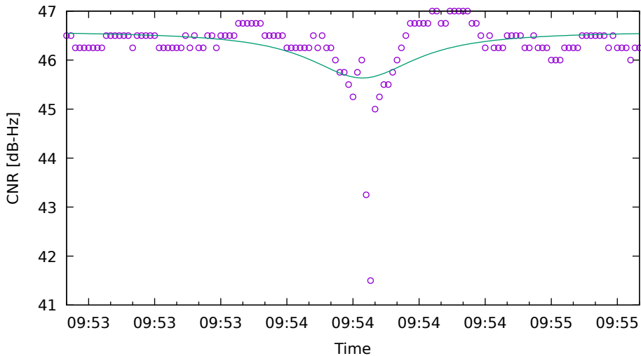
CNR fit for C34 on SamsungS20 - drive 9 (DOY263)
