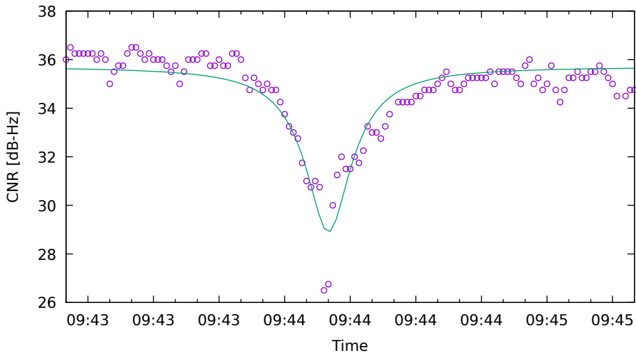
CNR fit for E12 on SamsungS20 - drive 3 (DOY263)
