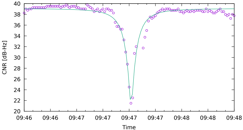
CNR fit for E12 on SamsungS20 - drive 5 (DOY263)
