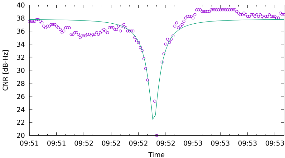
CNR fit for E12 on SamsungS20 - drive 8 (DOY263)
