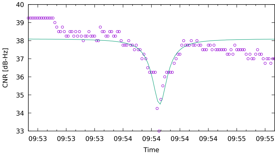
CNR fit for E12 on SamsungS20 - drive 9 (DOY263)
