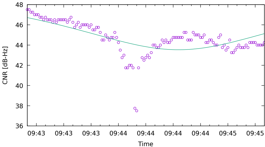
CNR fit for E33 on SamsungS20 - drive 3 (DOY263)
