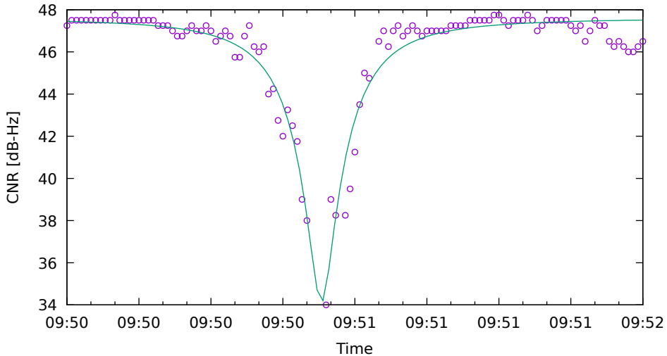
CNR fit for E33 on SamsungS20 - drive 7 (DOY263)
