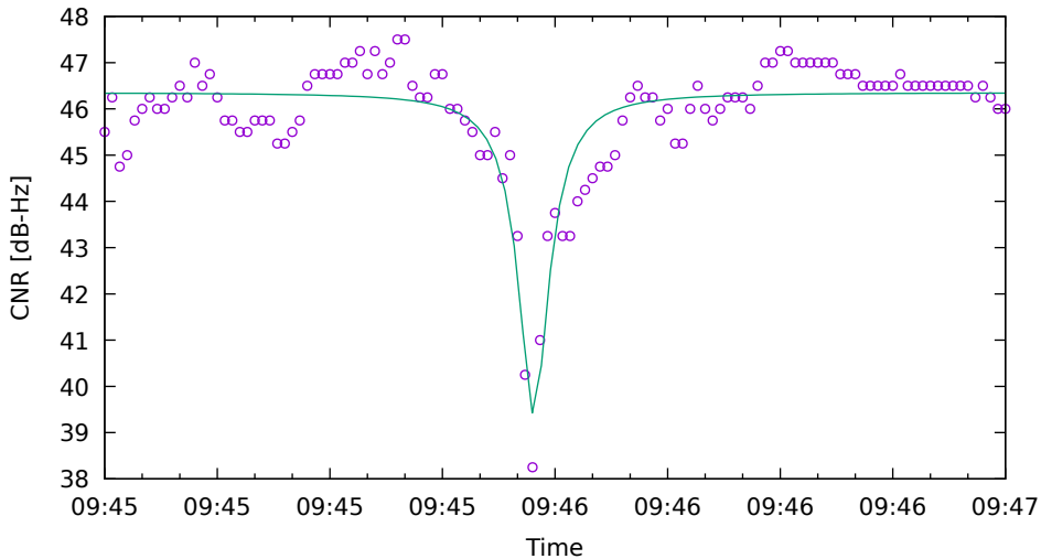
CNR fit for G01 on SamsungS20 - drive 4 (DOY263)
