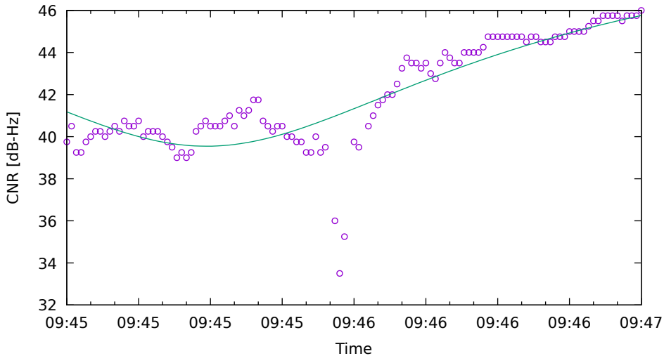
CNR fit for G03 on SamsungS20 - drive 4 (DOY263)
