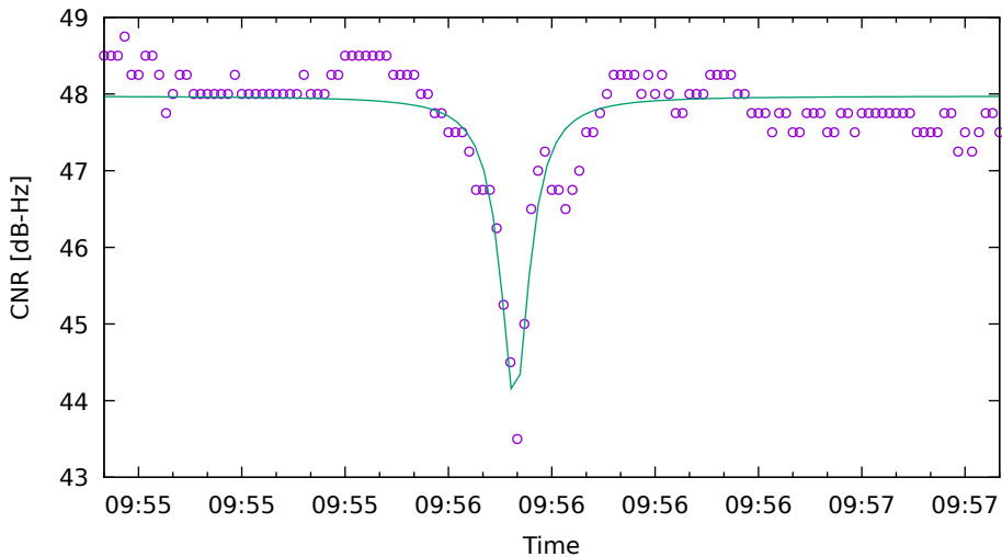
CNR fit for G04 on SamsungS20 - drive 10 (DOY263)
