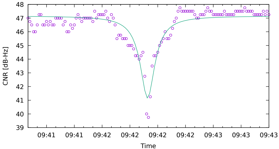
CNR fit for G04 on SamsungS20 - drive 2 (DOY263)
