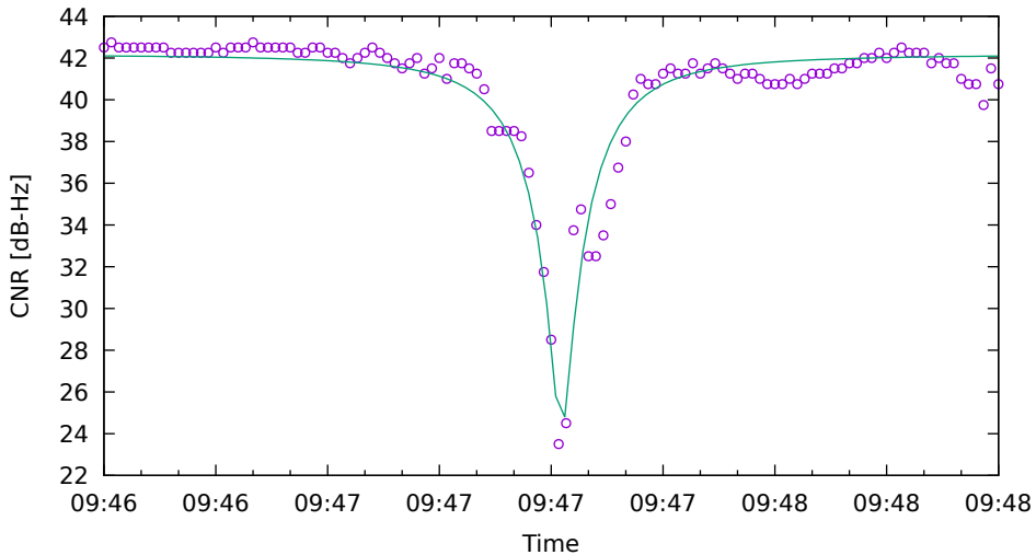
CNR fit for G08 on SamsungS20 - drive 5 (DOY263)
