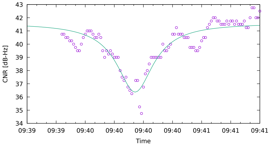
CNR fit for G17 on SamsungS20 - drive 1 (DOY263)
