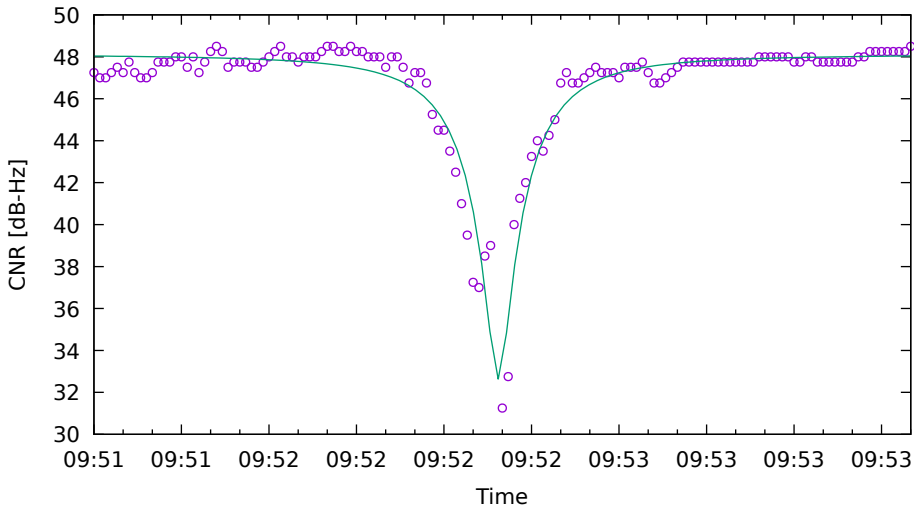
CNR fit for G17 on SamsungS20 - drive 8 (DOY263)
