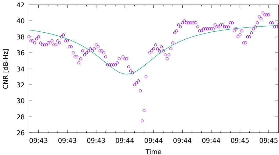
CNR fit for G32 on SamsungS20 - drive 3 (DOY263)
