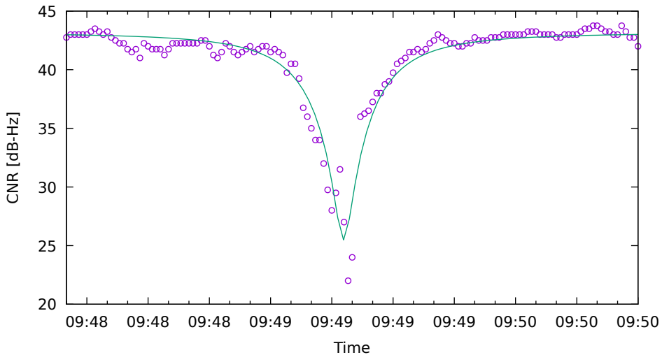
CNR fit for G32 on SamsungS20 - drive 6 (DOY263)
