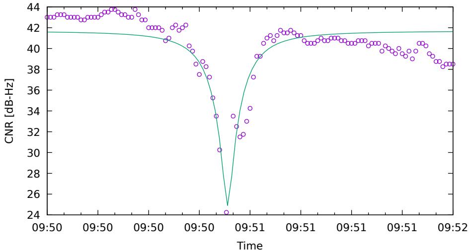
CNR fit for G32 on SamsungS20 - drive 7 (DOY263)
