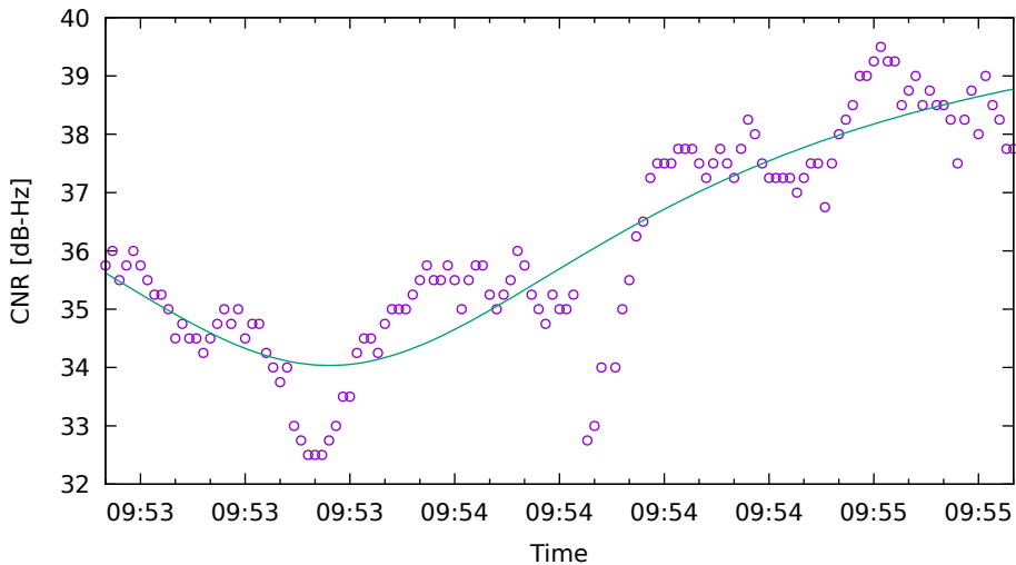
CNR fit for G32 on SamsungS20 - drive 9 (DOY263)
