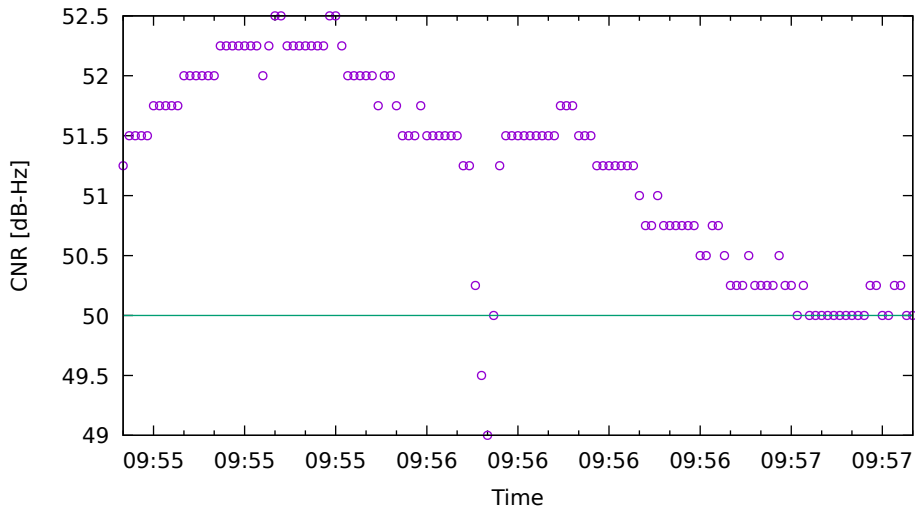
CNR fit for R02 on SamsungS20 - drive 10 (DOY263)
