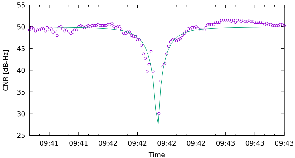
CNR fit for R02 on SamsungS20 - drive 2 (DOY263)
