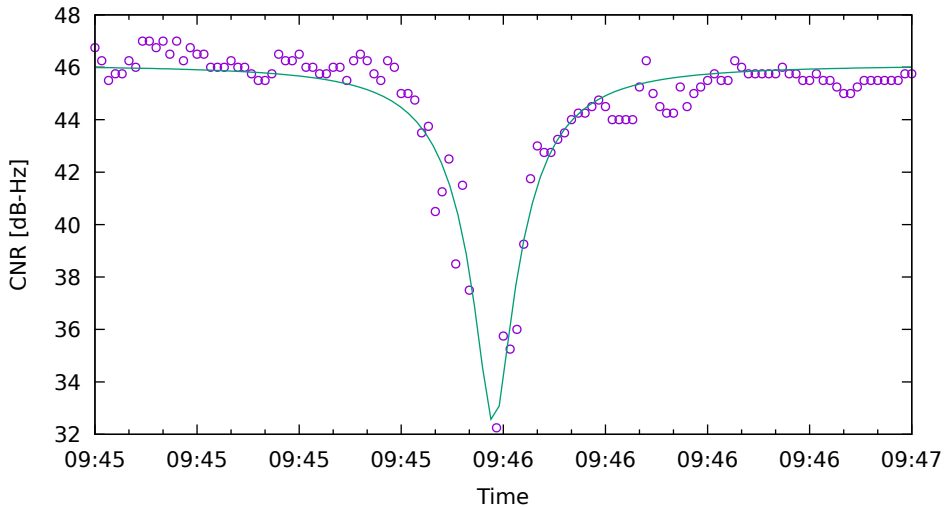
CNR fit for R02 on SamsungS20 - drive 4 (DOY263)
