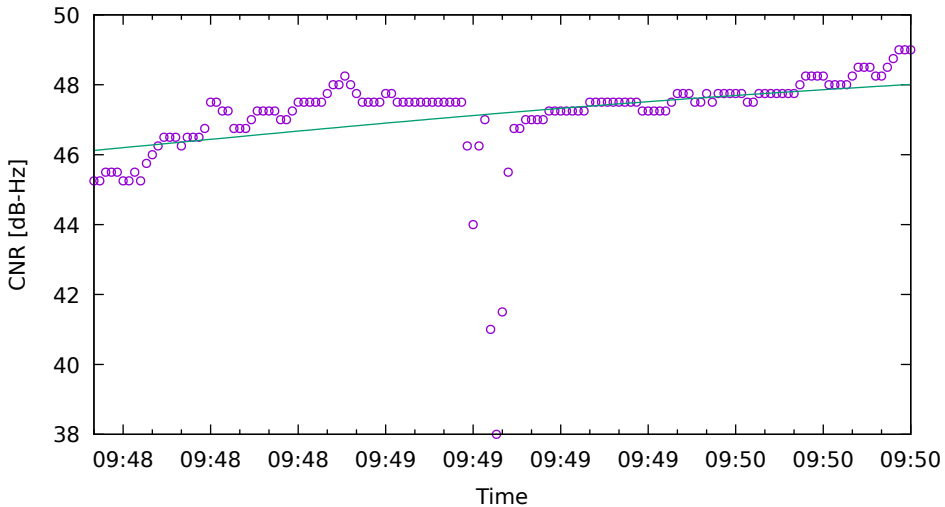
CNR fit for R02 on SamsungS20 - drive 6 (DOY263)
