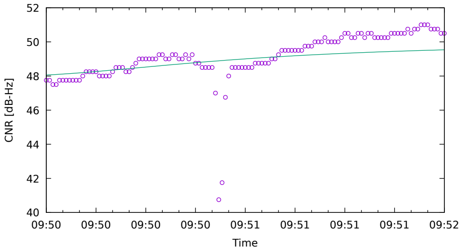
CNR fit for R02 on SamsungS20 - drive 7 (DOY263)
