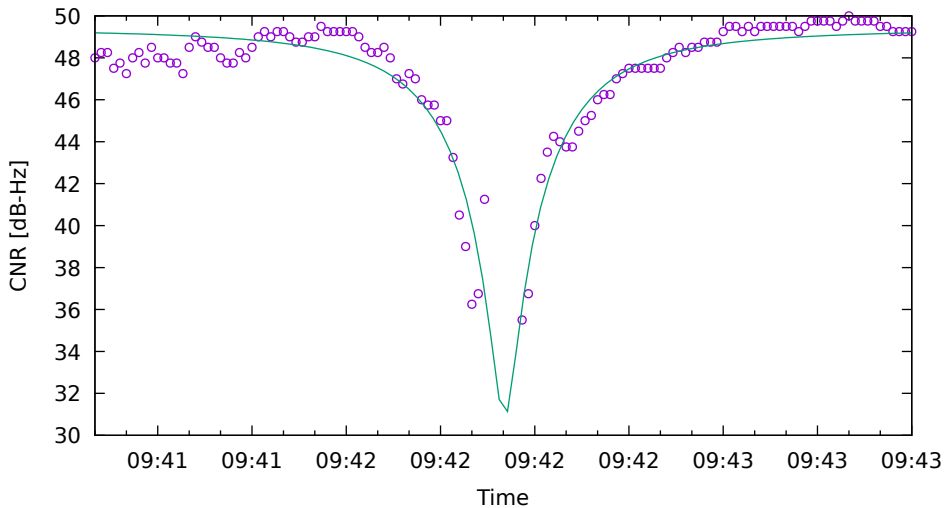
CNR fit for R17 on SamsungS20 - drive 2 (DOY263)
