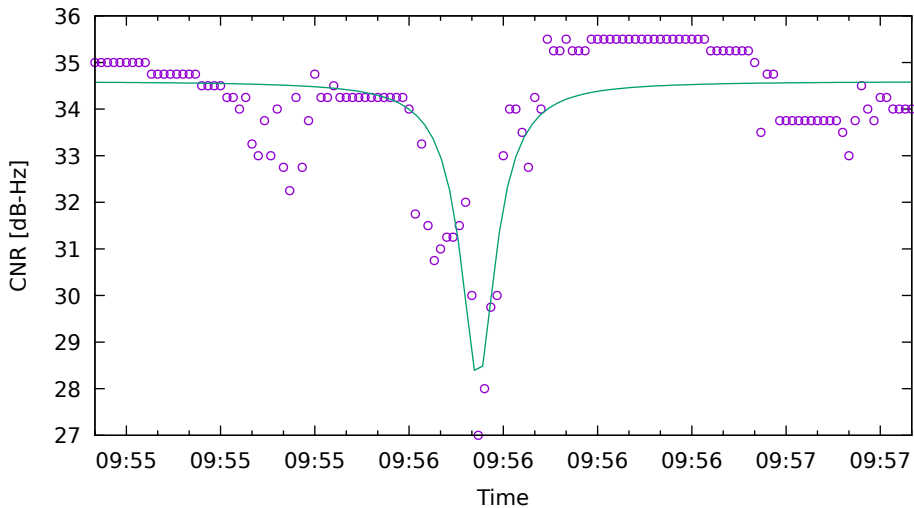
CNR fit for E04 on Xiaomi11T - drive 10 (DOY263)
