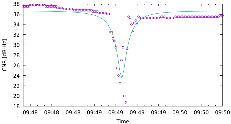
CNR fit for E04 on Xiaomi11T - drive 6 (DOY263)
