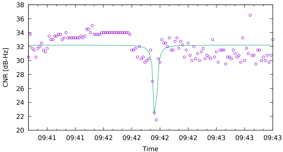
CNR fit for E11 on Xiaomi11T - drive 2 (DOY263)
