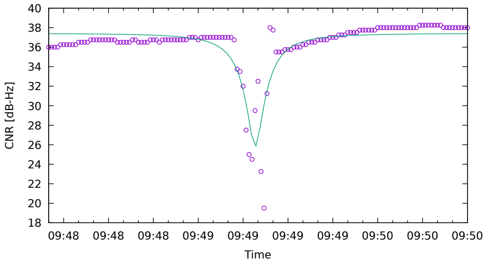
CNR fit for E11 on Xiaomi11T - drive 6 (DOY263)
