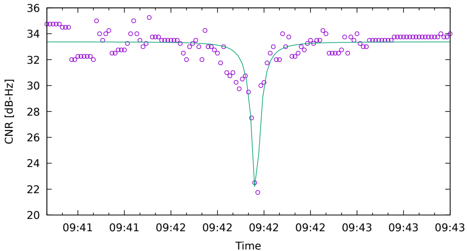
CNR fit for E12 on Xiaomi11T - drive 2 (DOY263)
