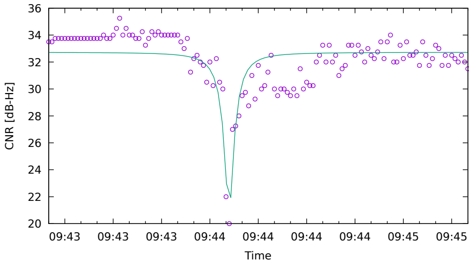
CNR fit for E12 on Xiaomi11T - drive 3 (DOY263)
