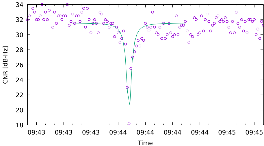
CNR fit for E19 on Xiaomi11T - drive 3 (DOY263)
