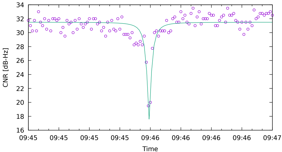
CNR fit for E19 on Xiaomi11T - drive 4 (DOY263)
