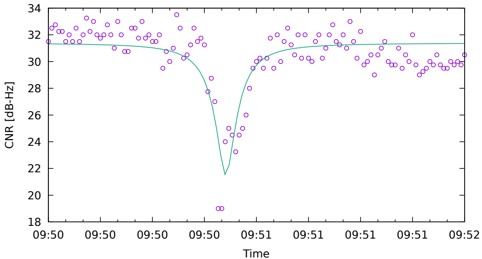
CNR fit for E19 on Xiaomi11T - drive 7 (DOY263)
