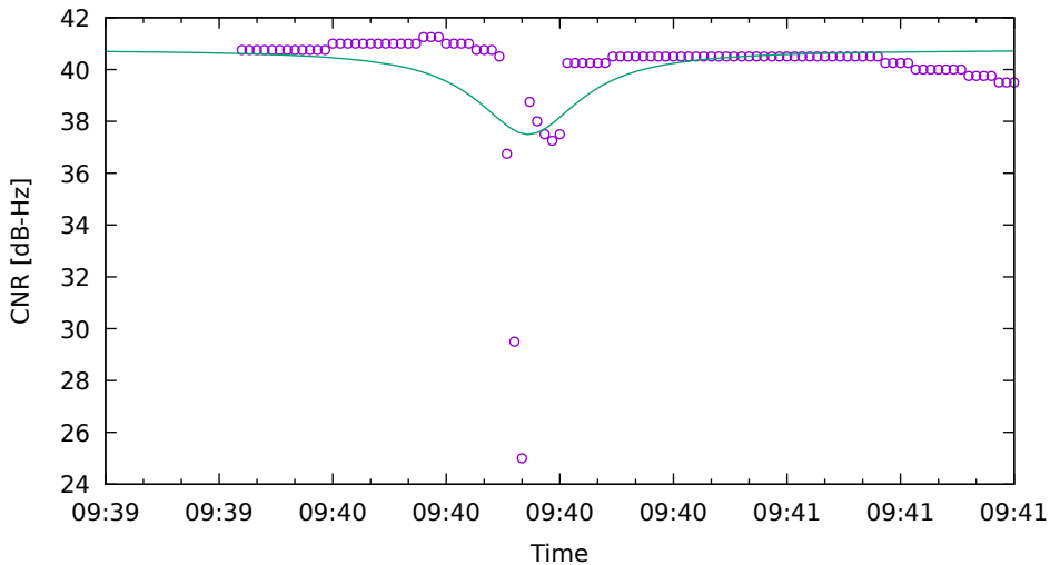
CNR fit for G01 on Xiaomi11T - drive 1 (DOY263)
