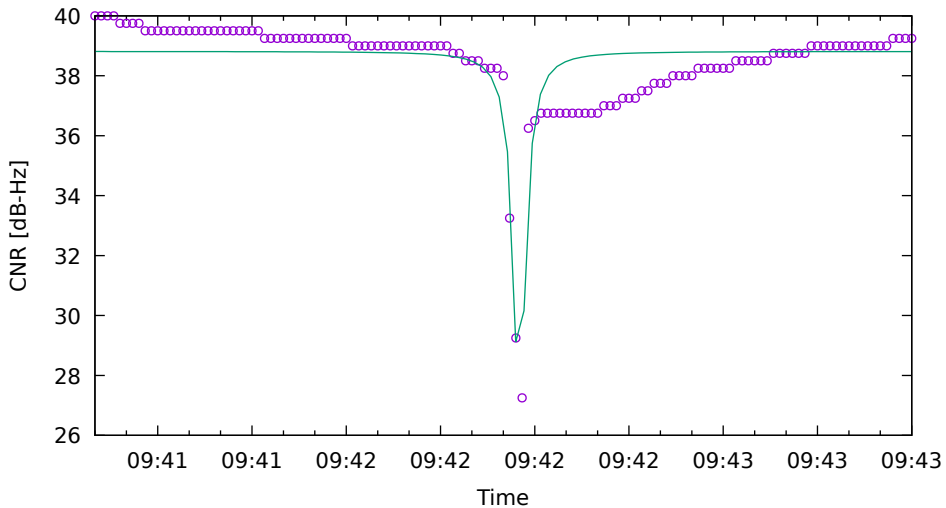
CNR fit for G01 on Xiaomi11T - drive 2 (DOY263)
