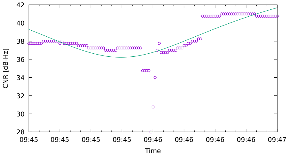
CNR fit for G01 on Xiaomi11T - drive 4 (DOY263)
