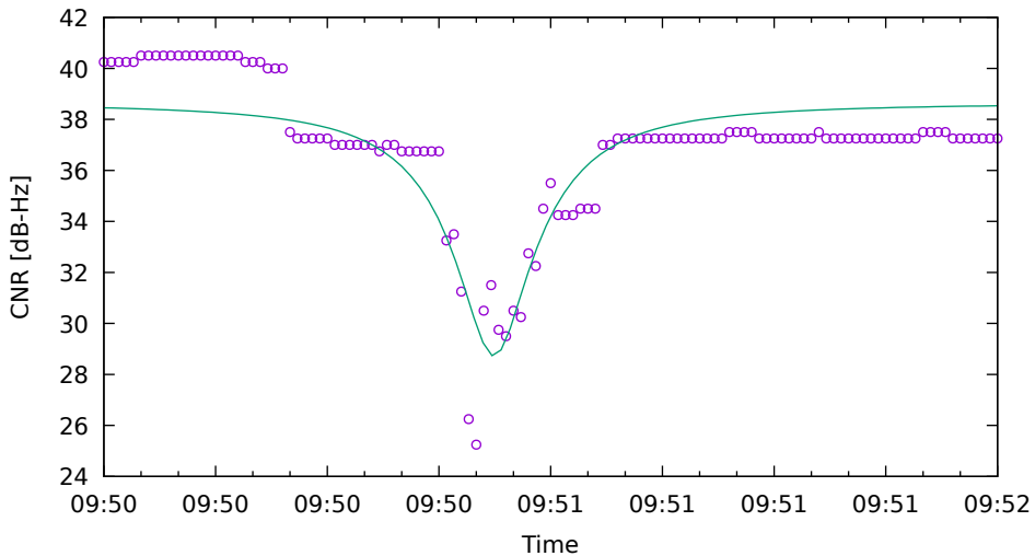
CNR fit for G01 on Xiaomi11T - drive 7 (DOY263)
