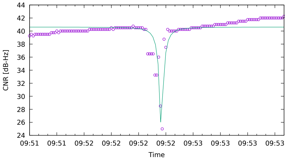
CNR fit for G03 on Xiaomi11T - drive 8 (DOY263)
