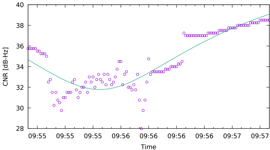
CNR fit for G17 on Xiaomi11T - drive 10 (DOY263)
