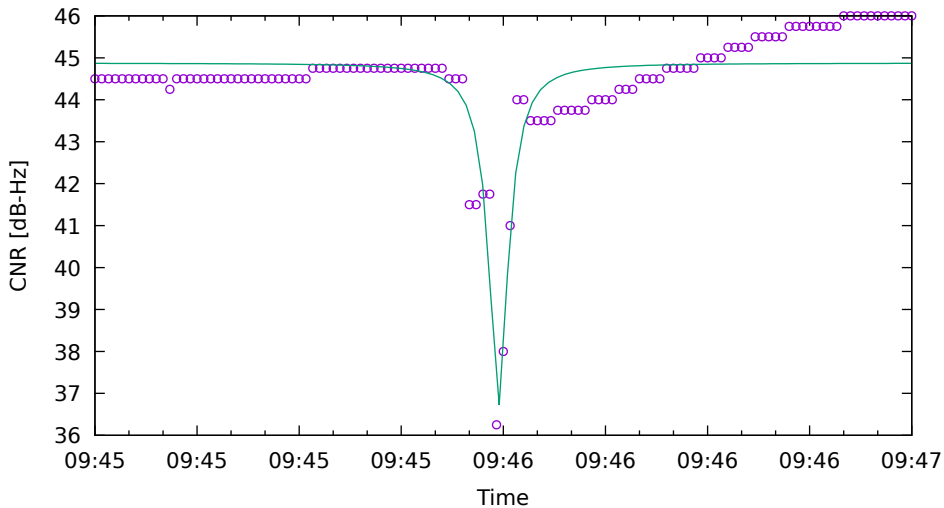
CNR fit for G22 on Xiaomi11T - drive 4 (DOY263)
