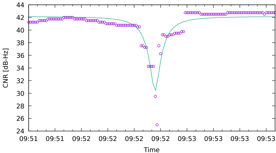
CNR fit for G22 on Xiaomi11T - drive 8 (DOY263)
